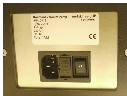
Rear Panel
